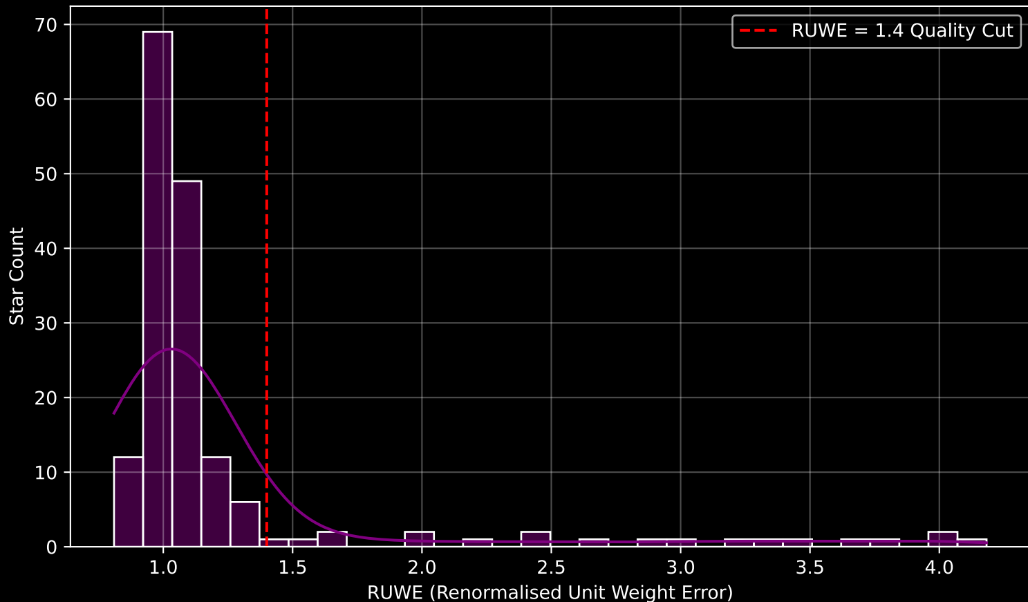
GAPOGEE DR17 Field [071+60_MGA] RUWE Distribution (n= 168)
