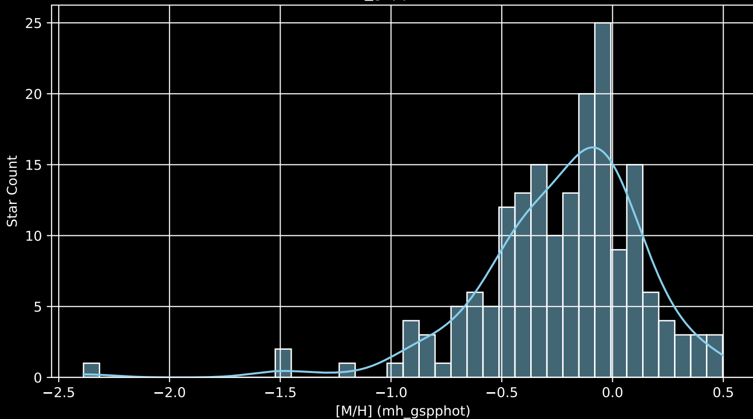
APOGEE DR17 Field: [071+60_MGA [M/H] (mh_gspphot) (n= 180)
