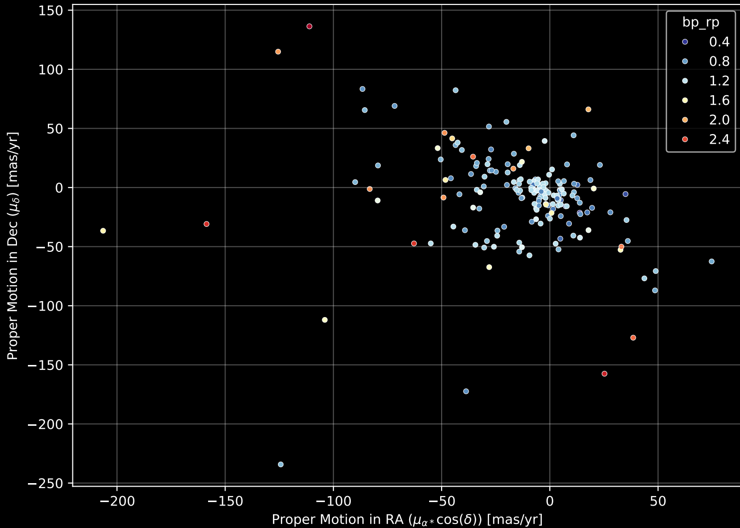
APOGEE DR17 Field: [071+60_MGA] Proper Motion Diagram (n= 181)
