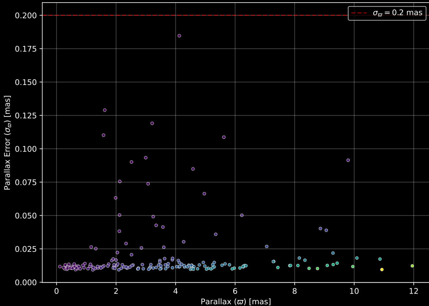
APOGEE DR17 Field: [071+60_MGA] Parallax Quality (n= 181)
