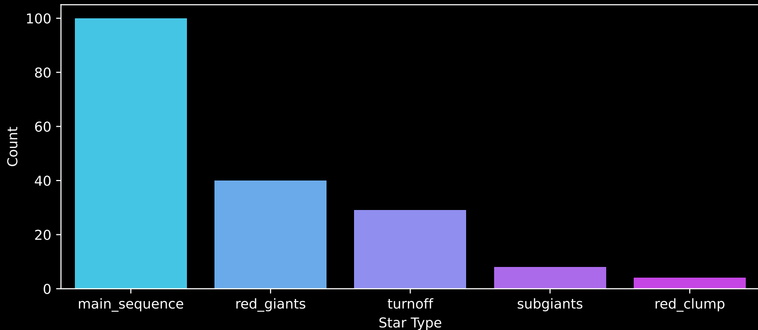
APOGEE DR17 Field: [071+60_MGA] Count plot of Star Type
