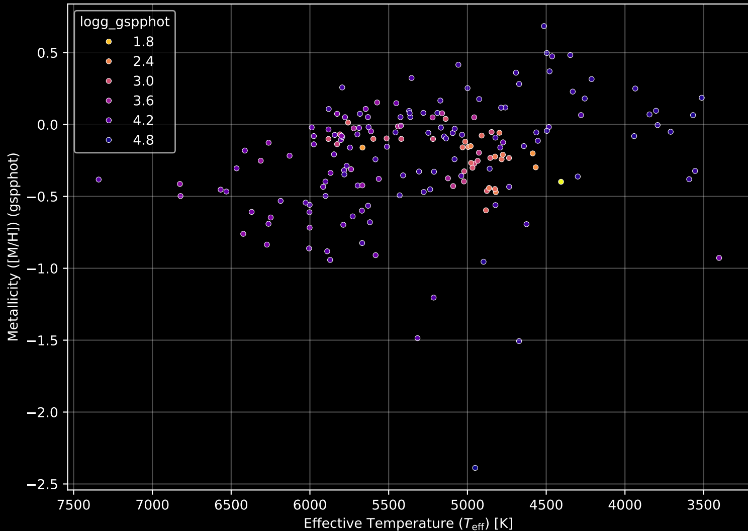
APOGEE DR17 Field: [071+60_MGA] Stellar Population Parameters (n= 181)
